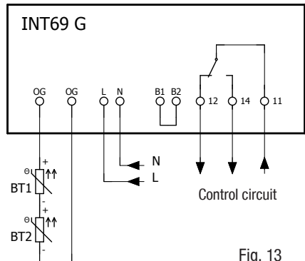
Fig. 13 Terminal box
